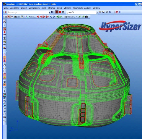
Image 3. HyperSizer software's structural sizing and design analysis of NASA's Composite Crew Module (CCM) enable the prediction of the structure's successful response to simulated flight condition load testing. This finite element model of the CCM displayed in HyperSizer shows the composite ply drops identified in green.
