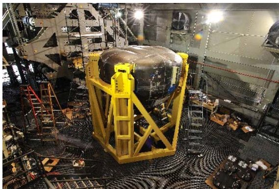
Image 4. NASA's Composite Crew Module (CCM) in the test rig (upside down) at NASA's Engineering and Safety Center (NESC) at Langley Research Center. The CCM project is being carried out to study materials tradeoffs between metals and composites in large space structures. Photo courtesy of NASA [EDITORS NOTE: A similar photo is also available in a vertical format]
